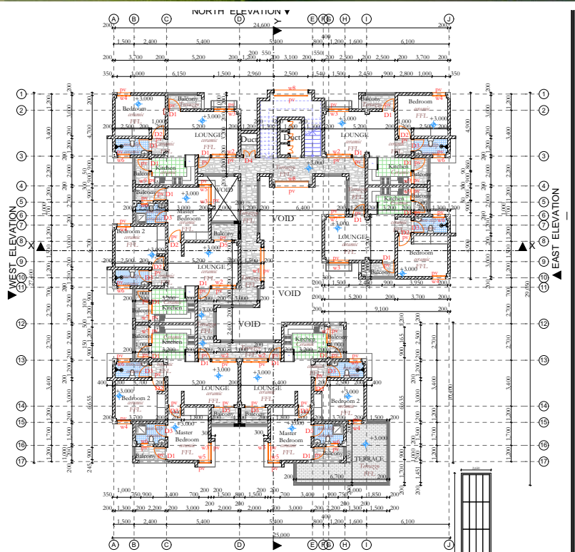
Floor plans
