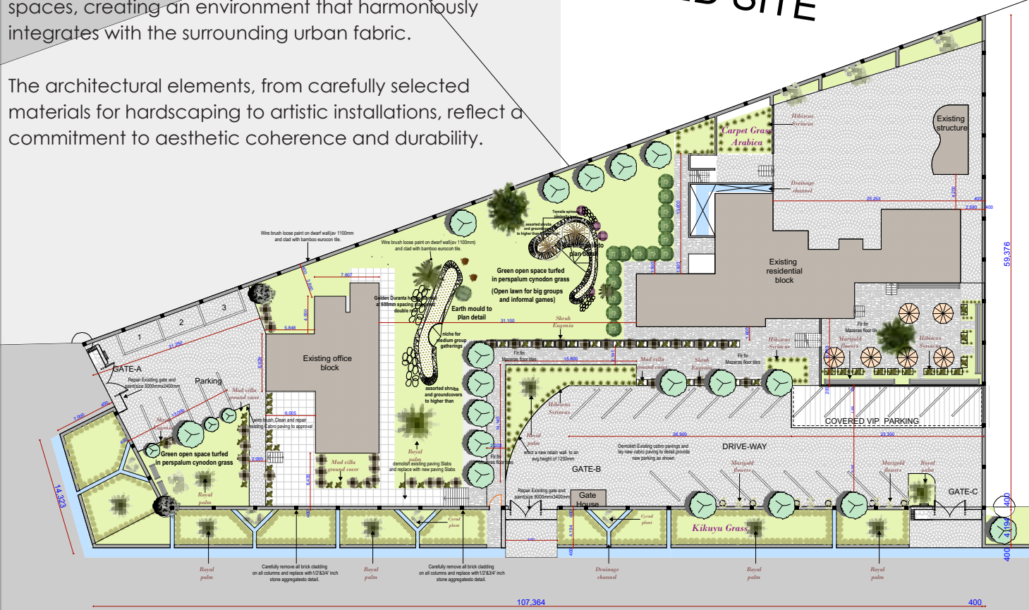
Masterplan
